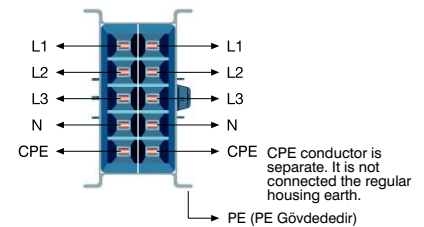
Feeder Box
